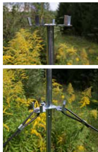
... mount the three bark beetle slit traps on the stand. Tip: Use pliers to bend and, thereby, slightly open hooks to facilitate installation.
