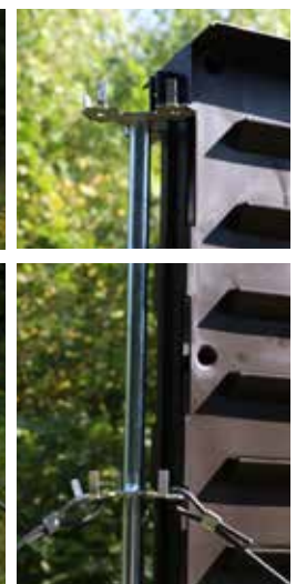
... mount the three bark beetle slit traps on the stand. Tip: Use pliers to bend and, thereby, slightly open hooks to facilitate installation.
